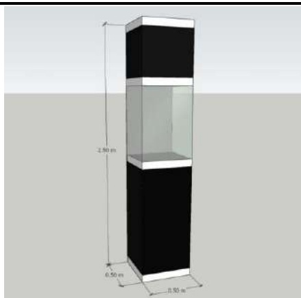
S1 - Tall Showcase A (W50xL50xH250 cm.)
