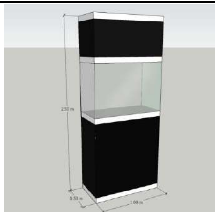
S2 - Tall Showcase B (W50xL100xH250 cm.)
